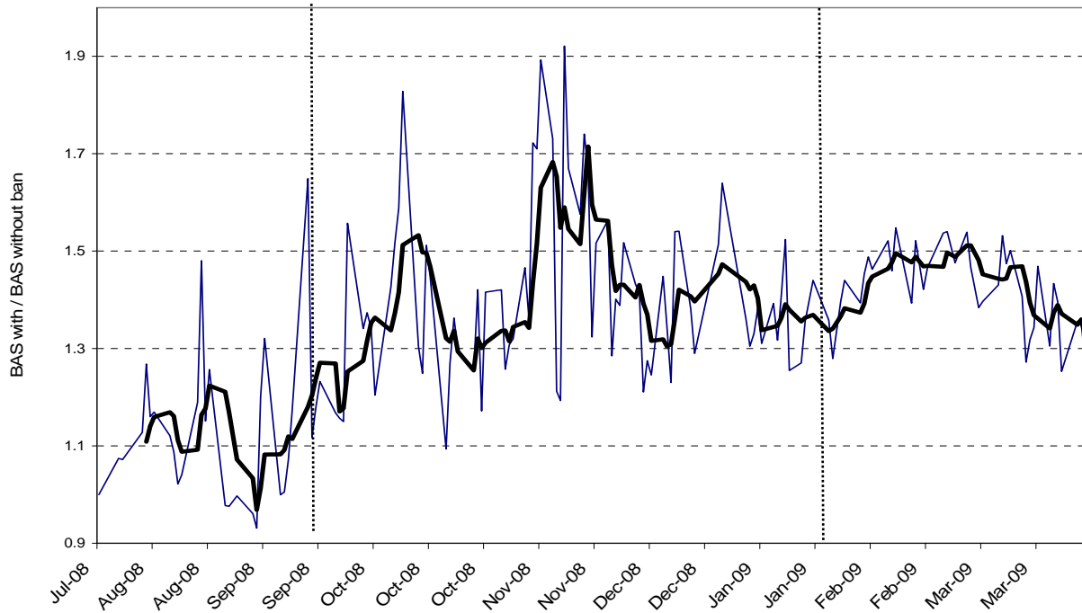
Figure A3. Ratio between Average Bid-Ask Spread for Stocks With and Without Ban in Switzerland and the U.K. (vertical lines: start and end of ban; thin line: daily values, bold line: 5-day moving average)
